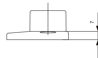
FOOTPLATE (TOP/BOTTOM)
