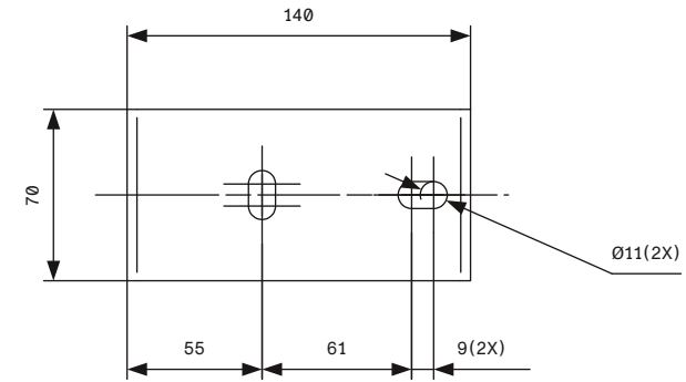
ROOF BRACKET: (VIEW A, FROM ABOVE)
